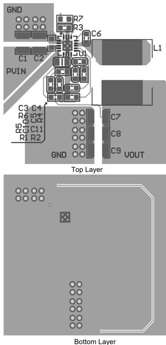
Figure 15. PCB Layout
