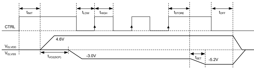
Figure 3. SGM3836B Programming V ELSS
