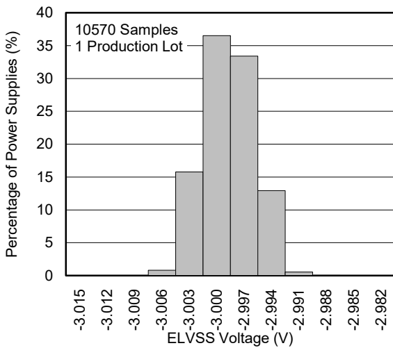
ELVSS (-3.0V) Voltage Production Distribution
