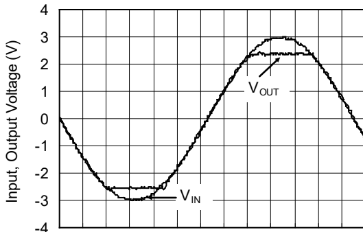
Time (5ms/div)
